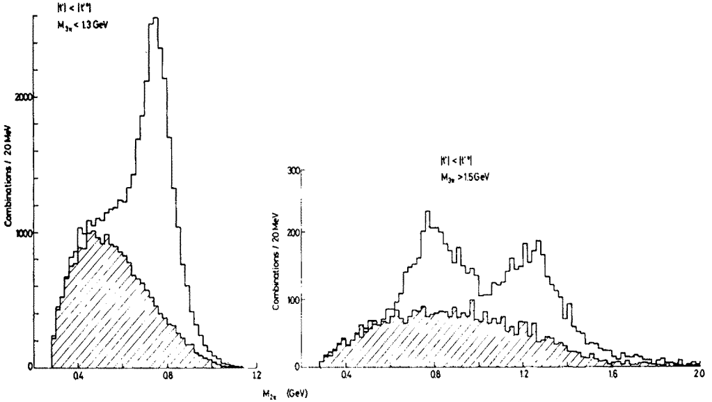
Fig. 12. 2\pi mass distribution for coherent events. The unshaded histograms are for the two \pi^+\pi^- combinations, the hatched ones for the \pi^+\pi^-\pi^- mass. The distributions are compiled for all target elements
