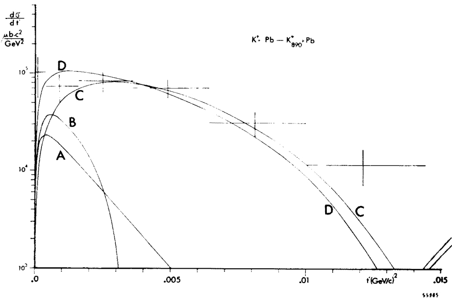
Fig. 32. Experimental and theoretical differential cross-sections for K^*(890) production on a Pb target. A : Coulomb, C : strong production, B : interference term (negative beyond 0.0032 (GeV/c) ^2 ). D : sum of A , B , C plus incoherent background. No t' dependence, but integrated cross-sections have been used in the fit resulting in curves A to D
